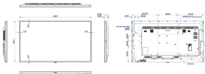
Philips 65BDL3050Q Type: 65BDL3050Q Model Year: 2019/2020
